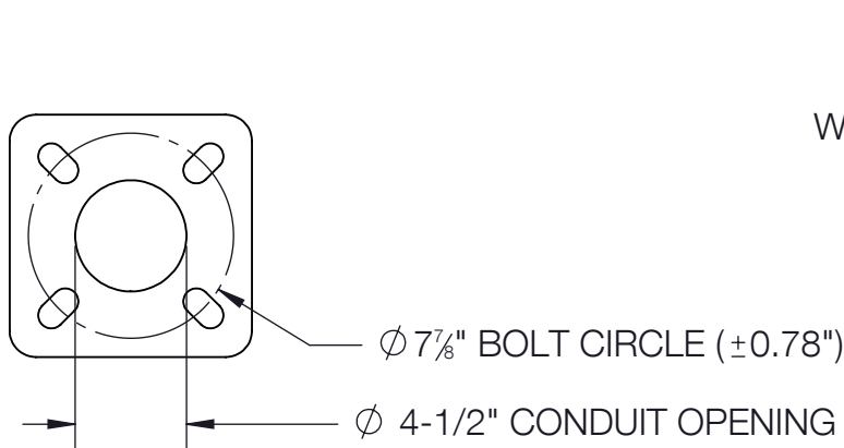
BASE DETAIL
