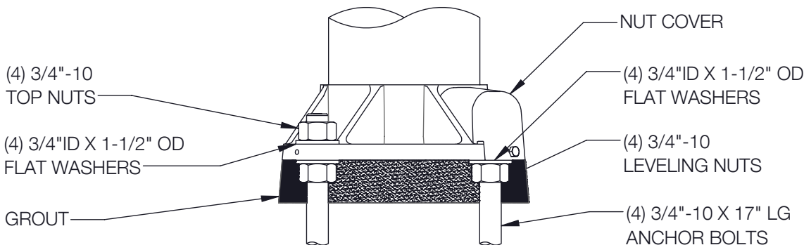
ANCHOR DETAIL
