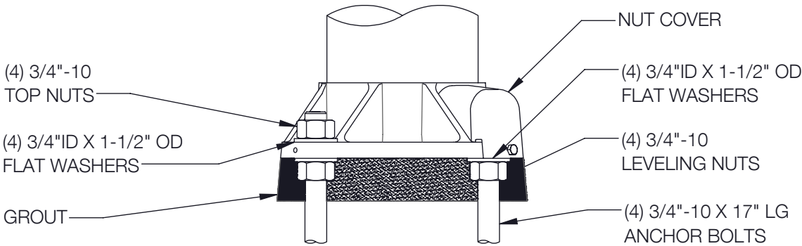
ANCHOR DETAIL
