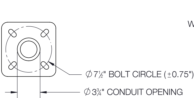
BASE DETAIL
