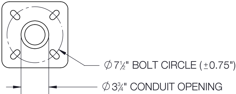
BASE DETAIL
