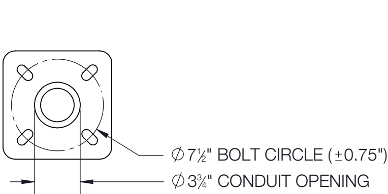
BASE DETAIL
