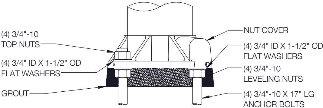
ANCHOR DETAIL
