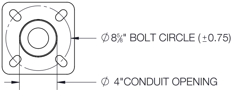
BASE DETAIL
