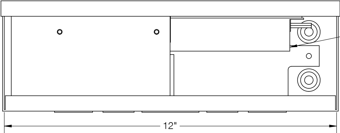
TOP VIEW (WITH COVER REMOVED)
