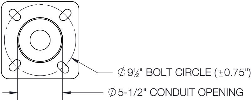
BASE DETAIL
