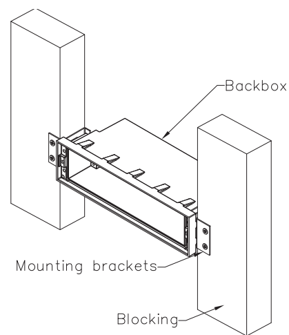
Figure 2 (stud wall)
