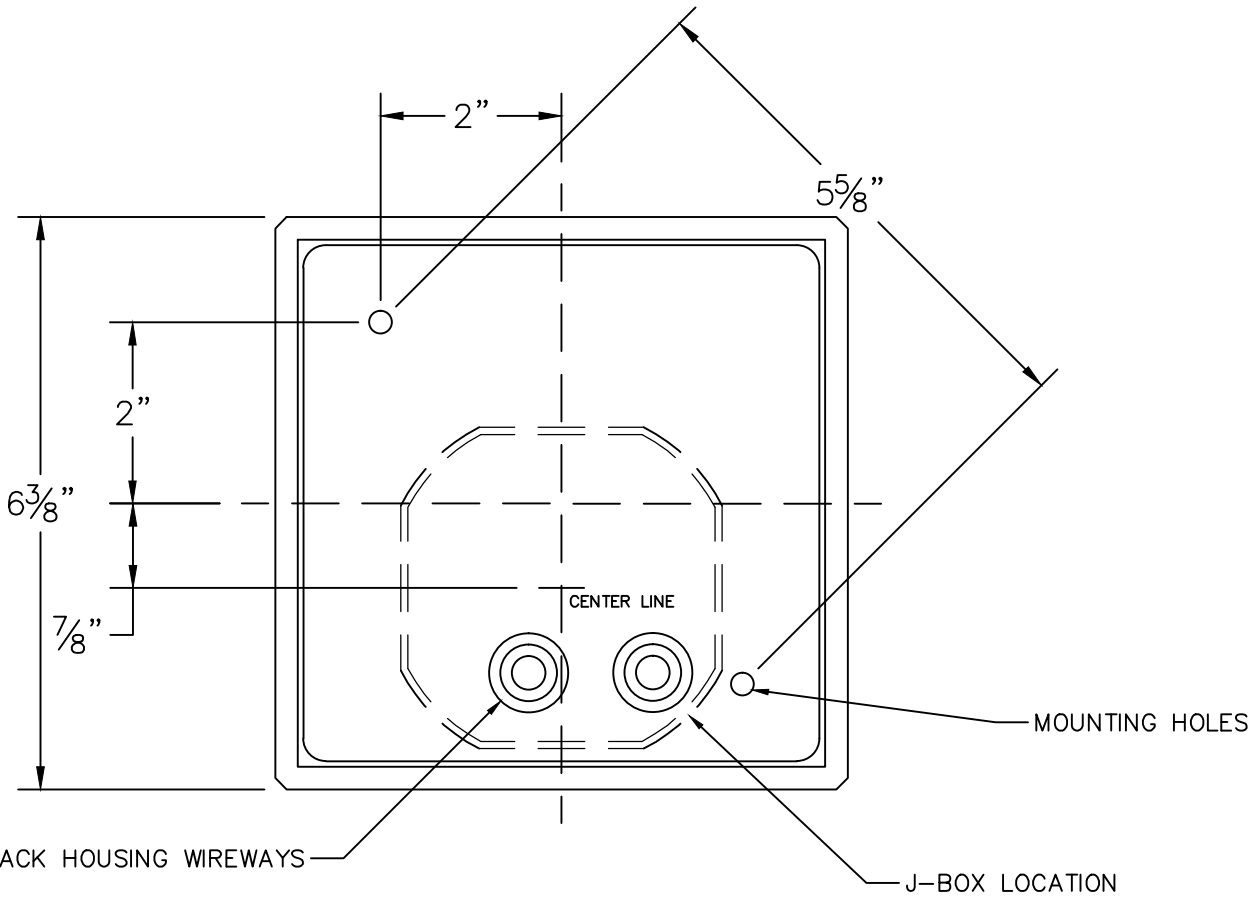
MOUNTING DETAIL
