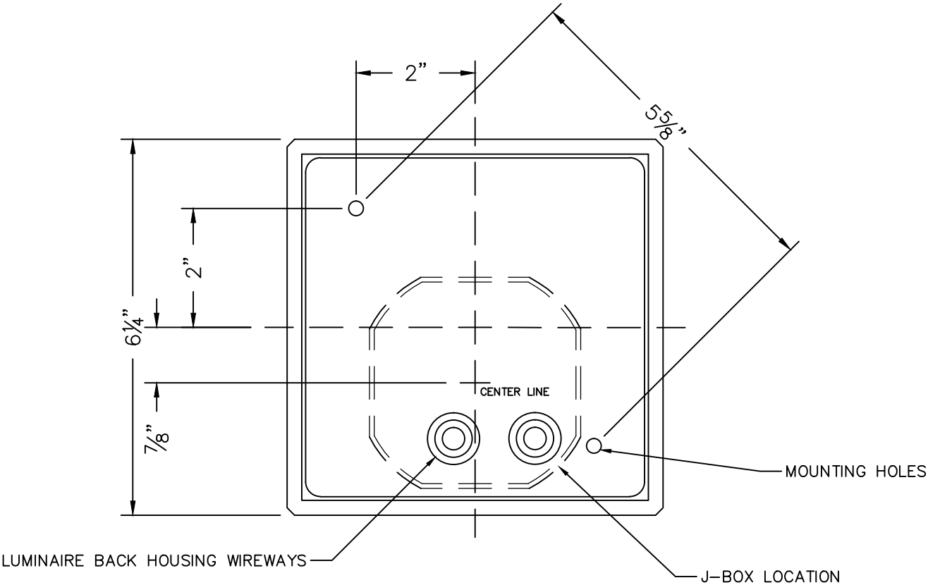
MOUNTING DETAIL
