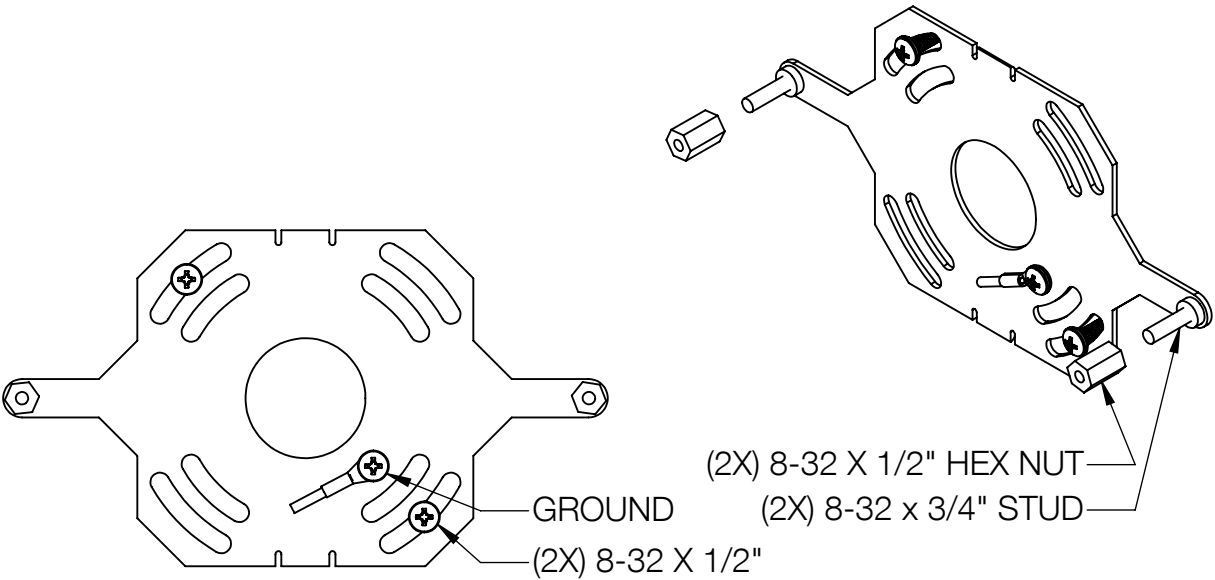
KIT #61 - DETAILS - MOUNTS DIRECTLY TO STANDARD OCTAGON BOX
