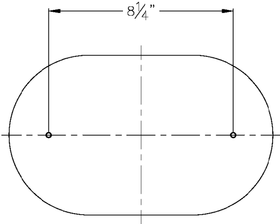
MOUNTING DETAIL
