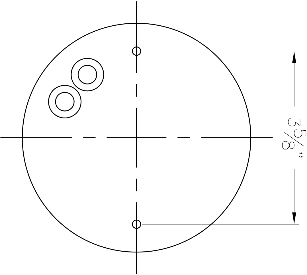
MOUNTING DETAIL
