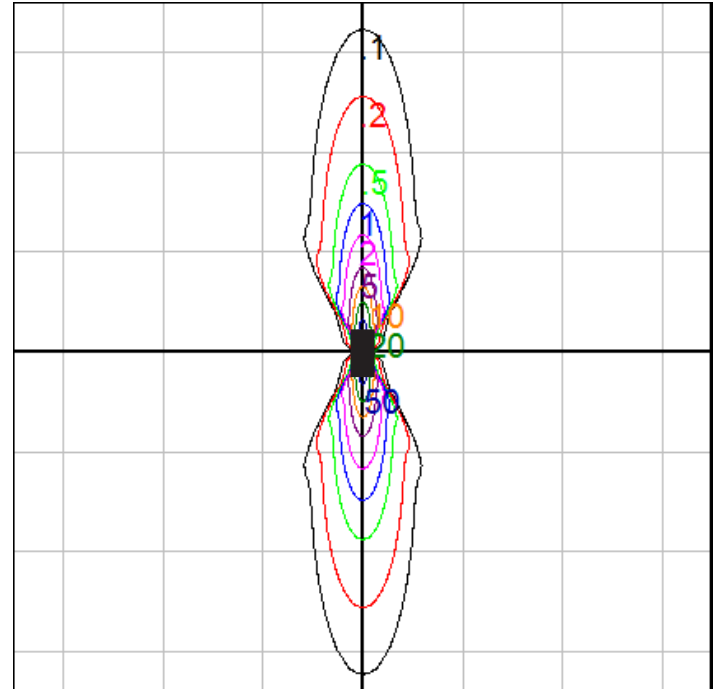
Wall mount fixture- Isofootcandle grid on wall Grid Spacing = 10 ft.
