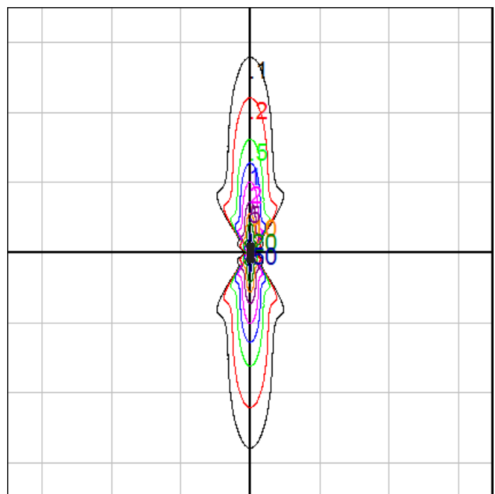
Wall mount fixture- Isofootcandle grid on wall Grid Spacing = 15 ft.
