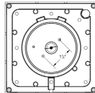
Figure 2: Luminaire back with round wall mount casting
