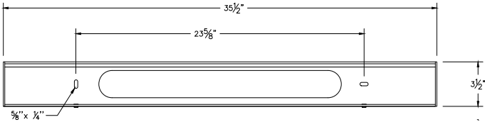
Figure 1: Mounting Detail
