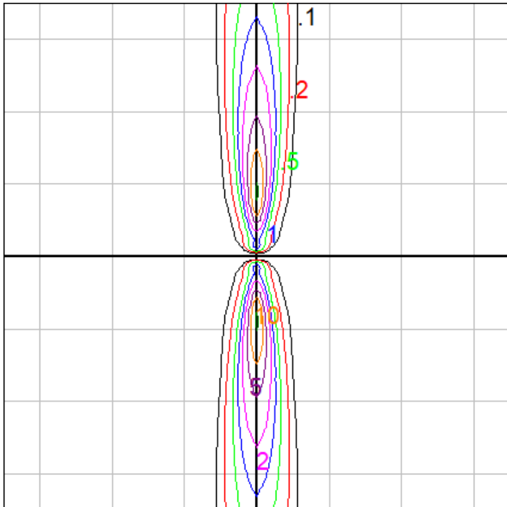
Grid Spacing: 3 ft. Isofootcandle grid on wall
