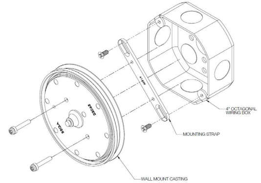
Figure 2: Luminaire back with round wall mount casting
