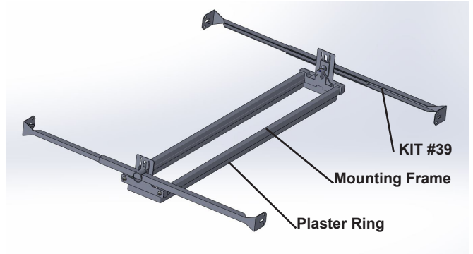
Figure 2 (Rough-in Kit with Plaster Ring Option)
