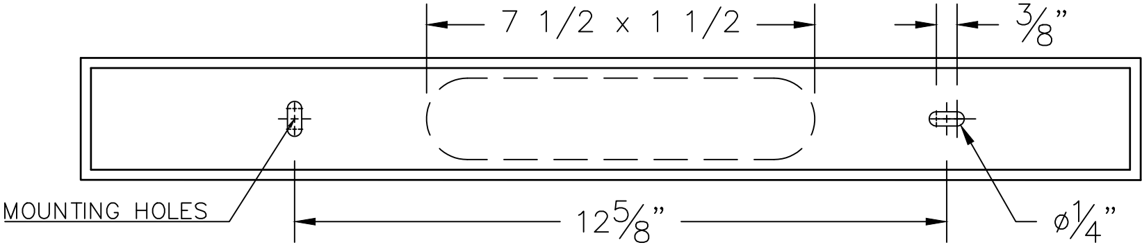
MOUNTING DETAIL
