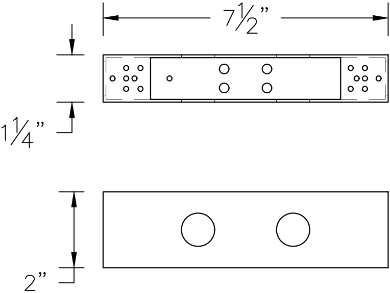
CUSTOM WIRING BOX DETAIL
