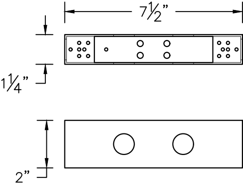
CUSTOM WIRING BOX DETAIL
