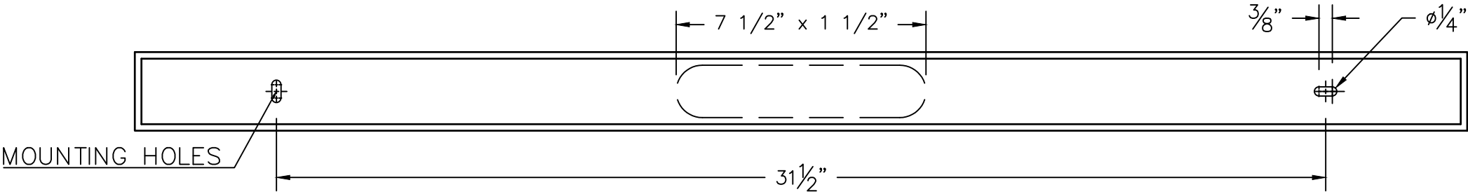
MOUNTING DETAIL
