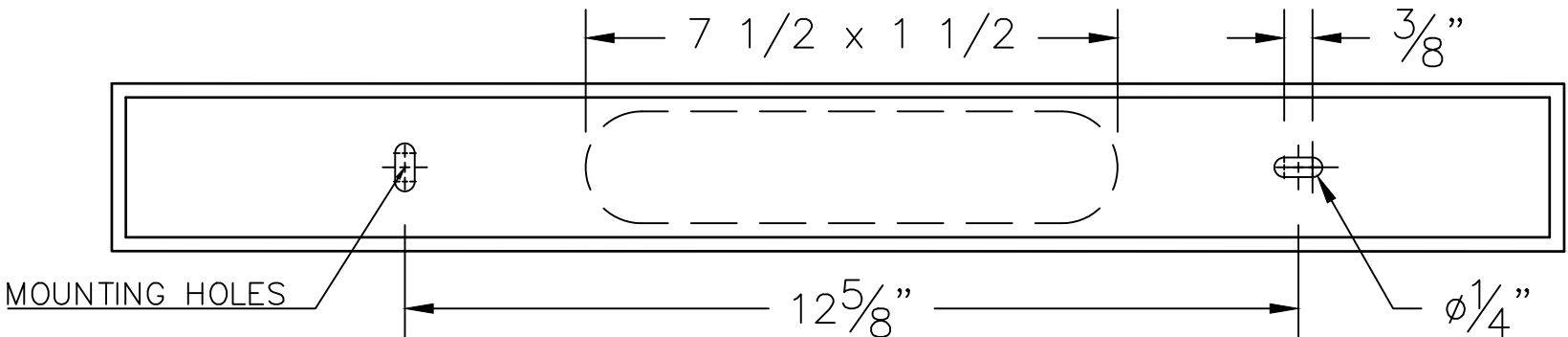
MOUNTING DETAIL
