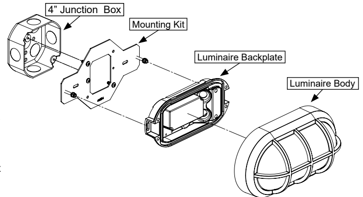
Figure 1: Mounting Diagram
