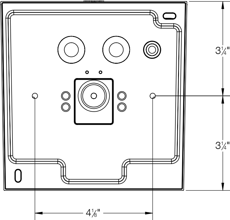
MOUNTING DETAIL
