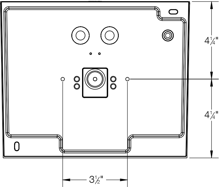
MOUNTING DETAIL
