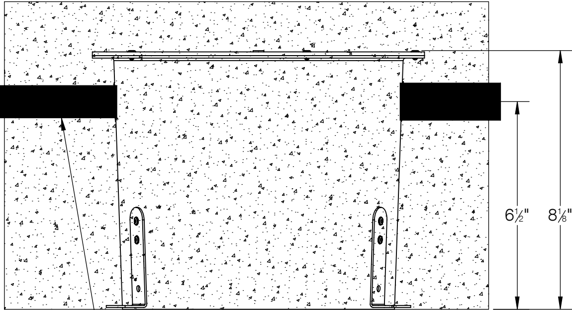
CONDUIT INSTALLATION HOUSING FOR CONCRETE CONSTRUCTION SHOWN BEFORE PLASTER RING INSTALLATION
