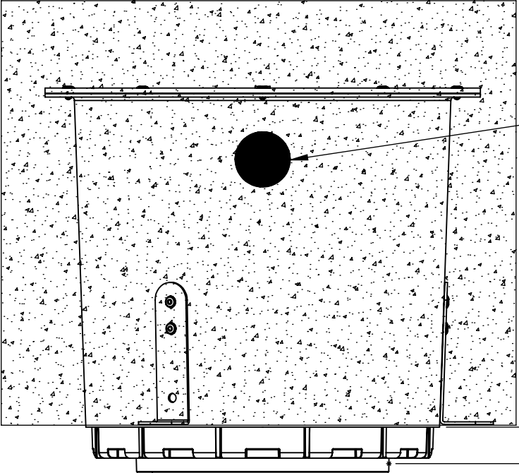
INSTALLATION HOUSING FOR CONCRETE CONSTRUCTION SHOWN WITH ADJUSTABLE PLASTER RING
