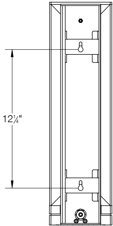
MOUNTING DETAIL
