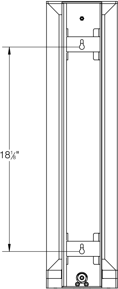
MOUNTING DETAIL
