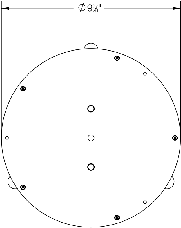
TOP VIEW
