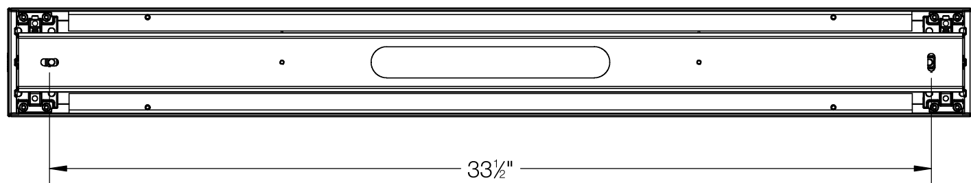
BACK VIEW (MOUNTING DETAIL)
