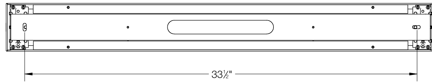
BACK VIEW (MOUNTING DETAIL)
