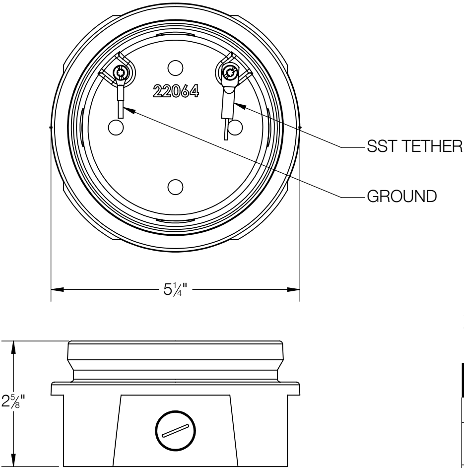
SURFACE WIRING BOX DETAILS
