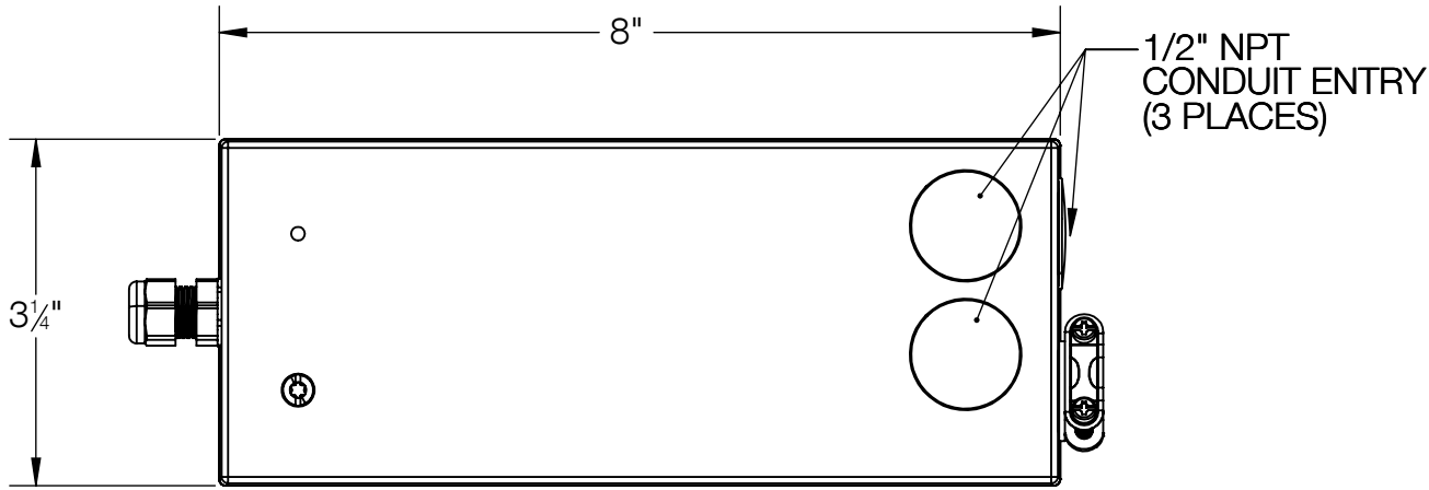
CEILINGBOX-L-11 (INCLUDED)
