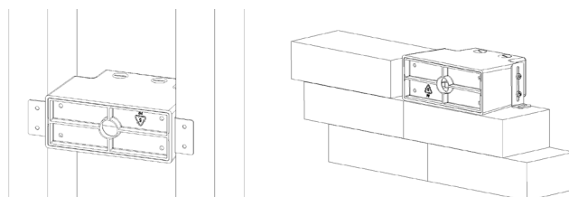
Figure 3: Poured concrete
