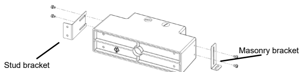
Figure 1: Included brackets
