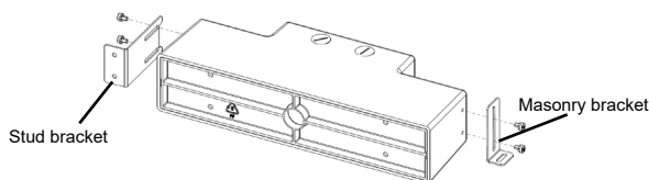
Figure 2a: Hollow (stud) wall
