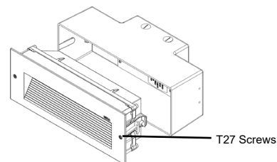
Figure 4: Installation
