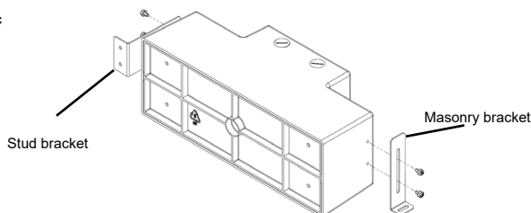
Figure 2a: Hollow (stud) wall
