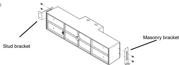
Figure 2a: Hollow (stud) wall
