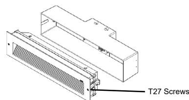
Figure 4: Installation
