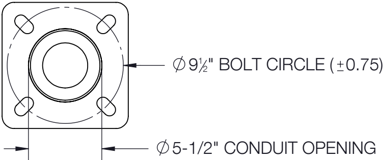
BASE DETAIL
