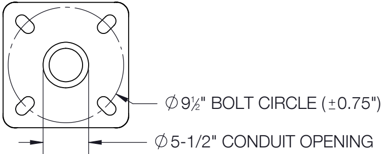
BASE DETAIL
