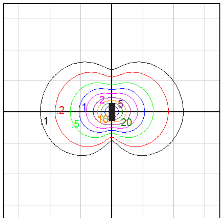
Wall Mount - Isogrid on Wall Grid Spacing = 5 ft.
