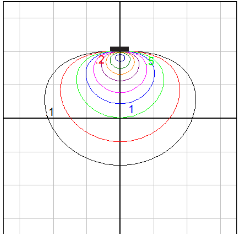
Wall Mount Fixture - Iso Grid on Wall Grid Spacing = 2 ft.
