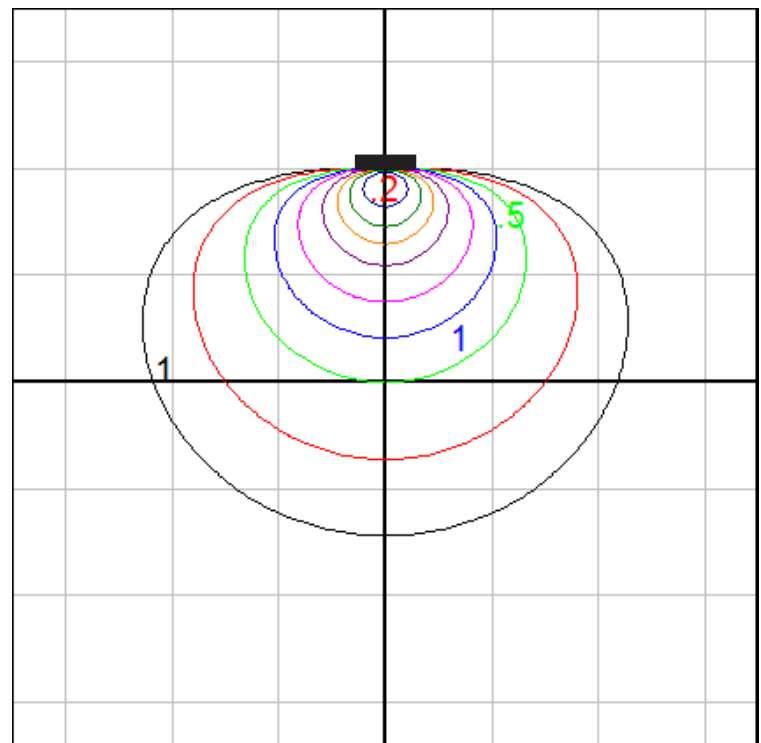
Wall Mount Fixture - Iso Grid on Wall Grid Spacing = 5 ft.
