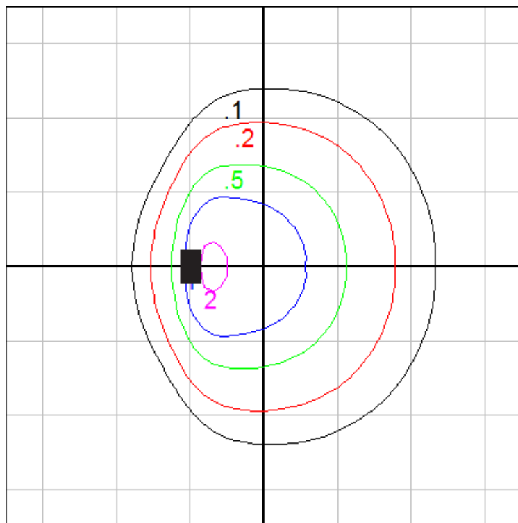
Wall Mount - Isofootcandle grid on floor Mounting Height = 20 ft. Grid Spacing = 15 ft.
