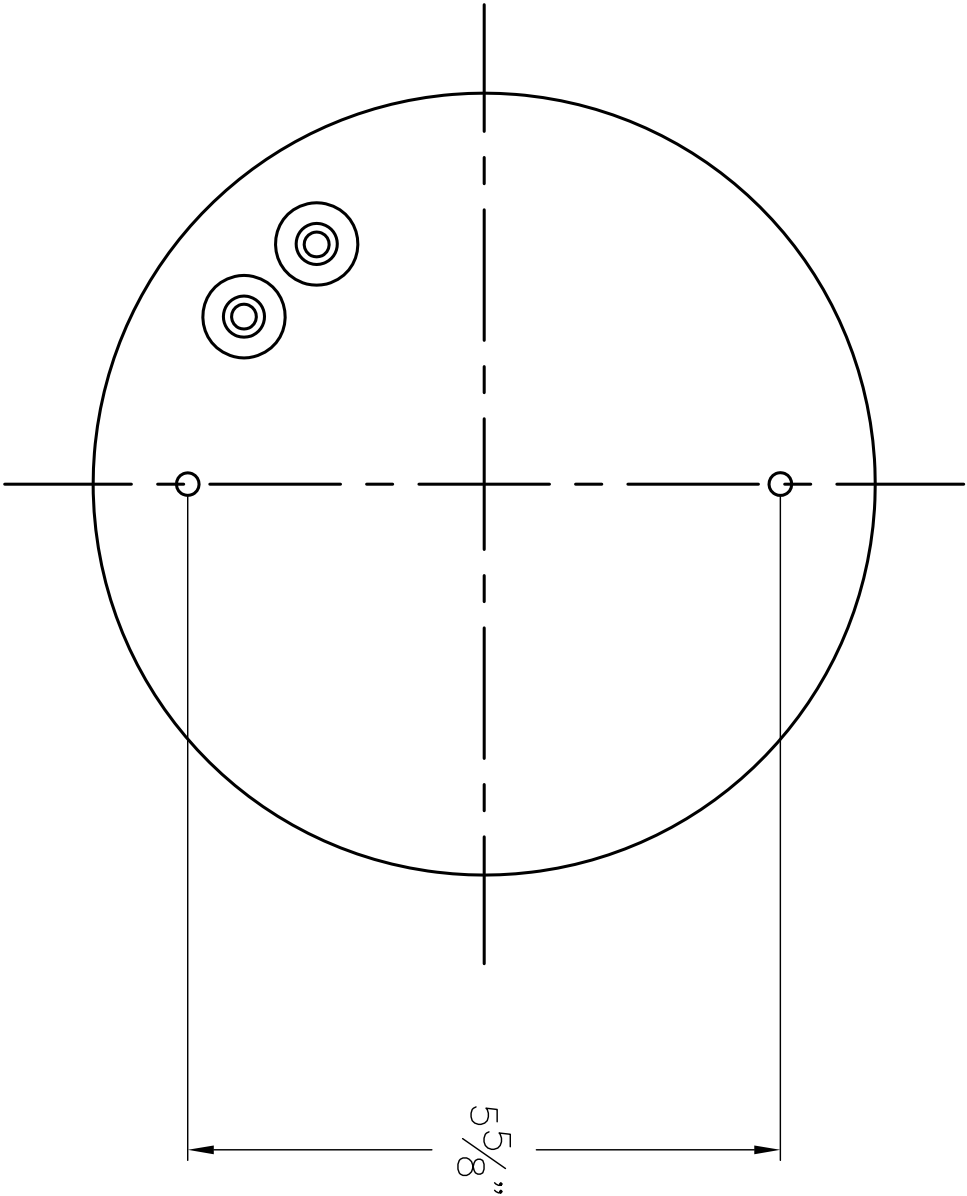
MOUNTING DETAIL
