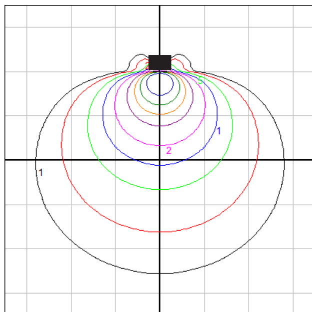
Grid Spacing = 2.5 ft. Isofootcandle grid on wall
