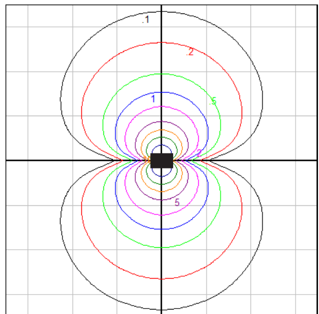
Grid Spacing = 2.5 ft. Isofootcandle grid on wall
